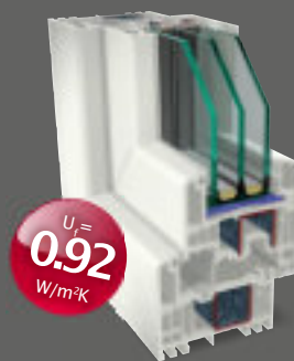
Narrow frame with sash and confirmed ift passive house-compatibility
